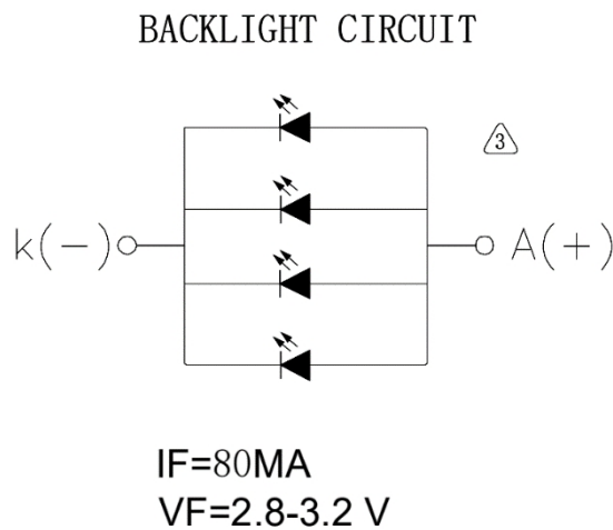
Fig.3*Schematics drawing of lighting (绘制照明图 图.3)
