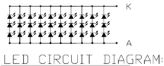
Fig.3*Schematics drawing of lighting (绘制照明图 图.3)
